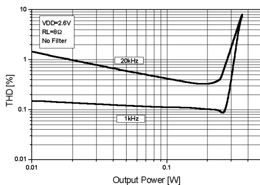
Figure 3. THD+N versus output power
