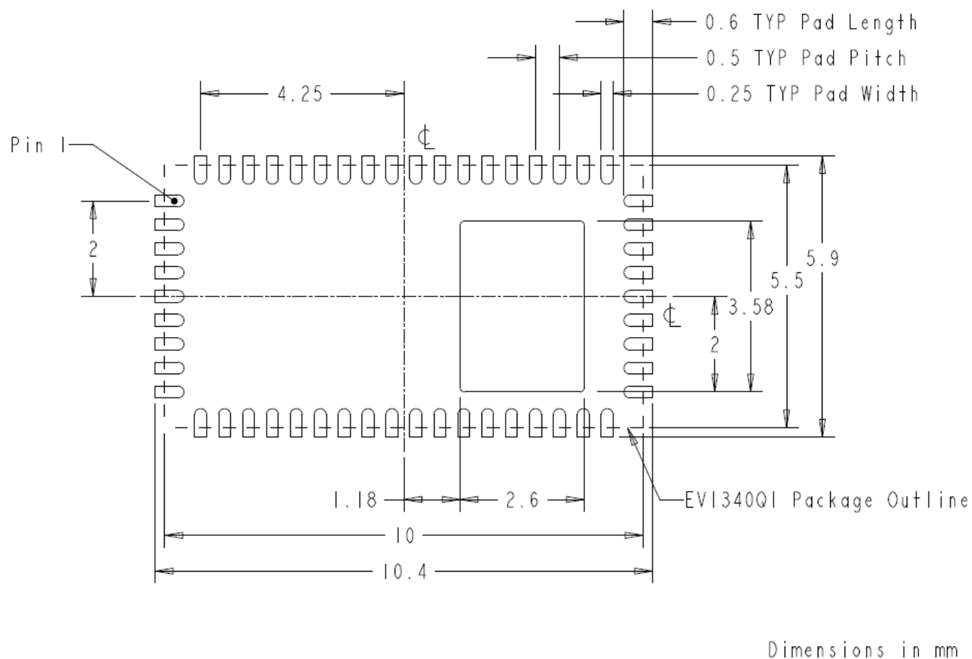
Figure 11: EV1340 Package PCB Footprint (Top View)
