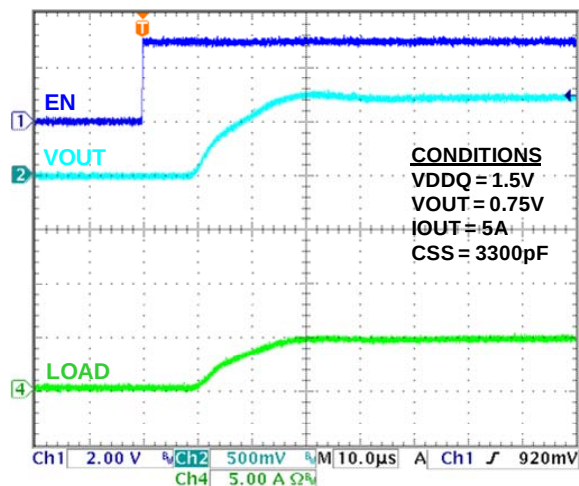
Startup with Enable
