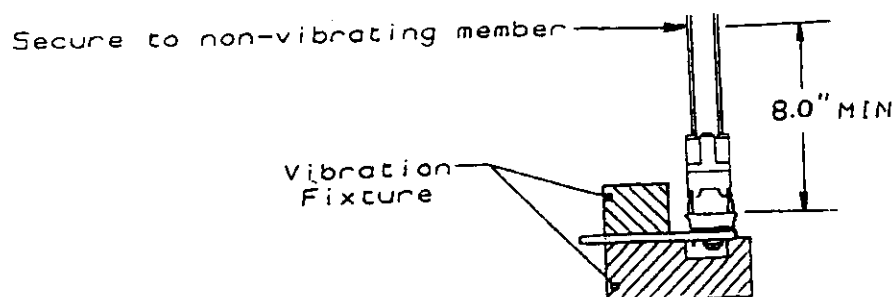
Figure 4 Vibration & Physical Shock Mounting Fixture
