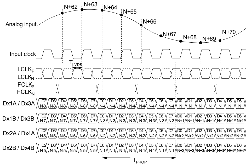
Figure 6: Dual channel - LVDS timing 8-bit output
