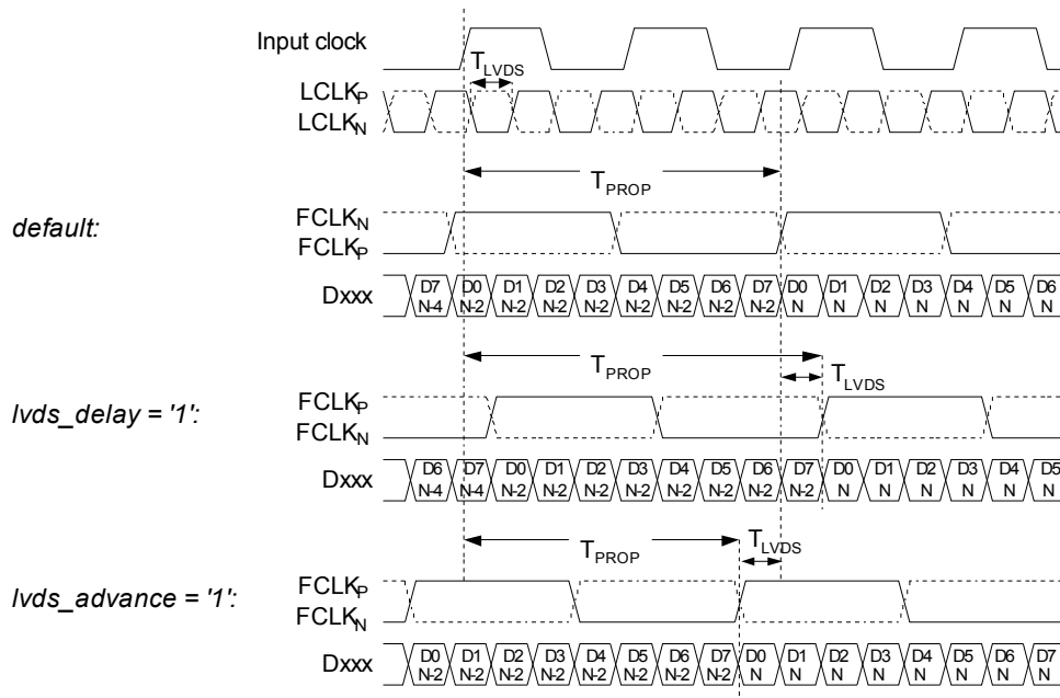
Figure 10: LVDS output timing adjustment
