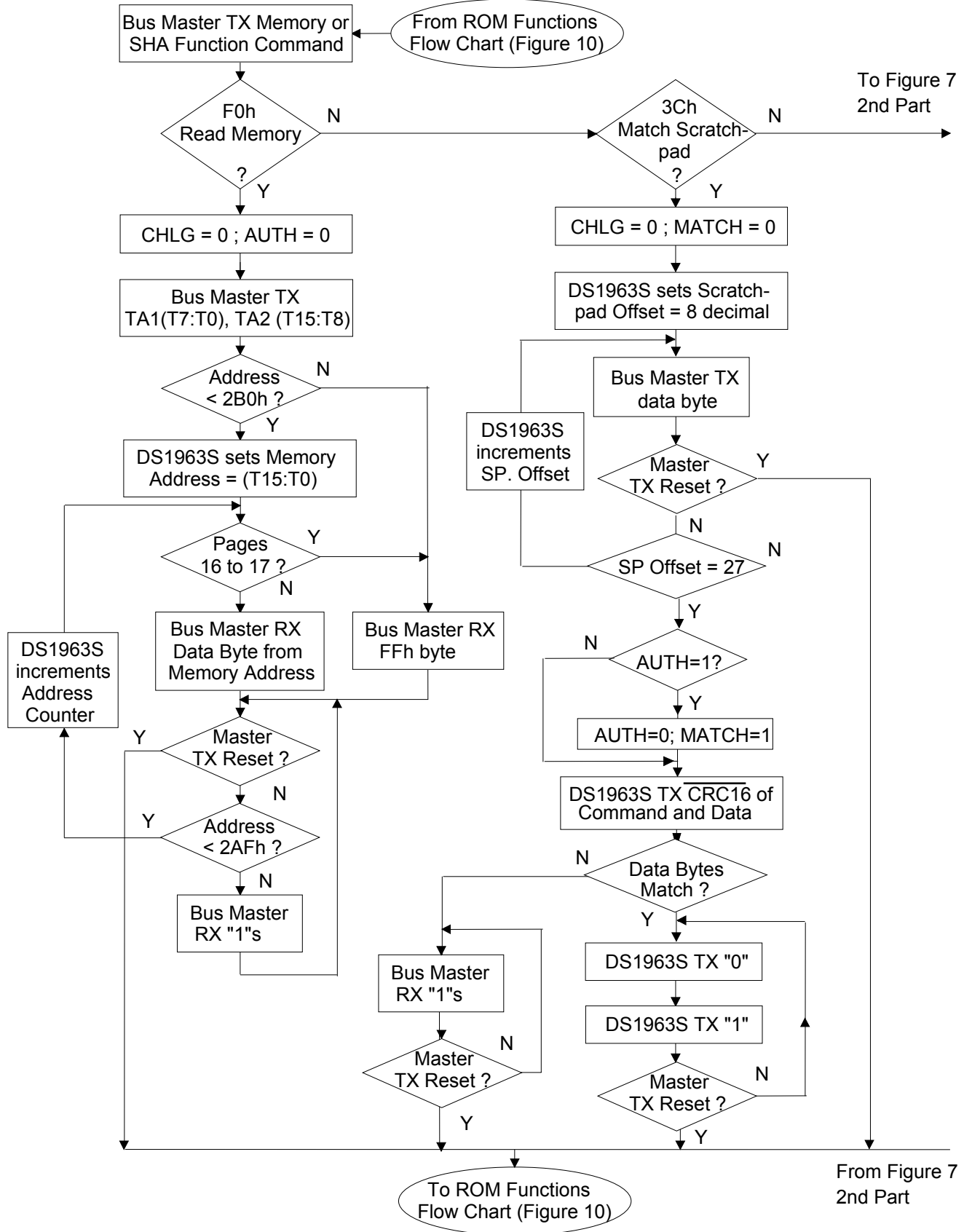
Memory and SHA Function Flow Chart Figure 7
