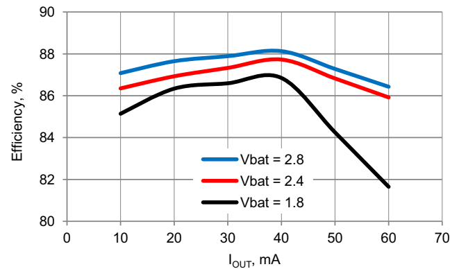
Figure 11-9. Efficiency vs I OUT V BOOST = 3.3 V, L BOOST = 22 µH [29]
