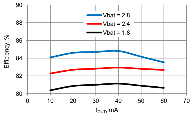
Figure 11-8. Efficiency vs I OUT V BOOST = 3.3 V, L BOOST = 10 µH [29]
