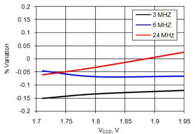
Figure 11-60. IMO Frequency Variation vs. V CC
