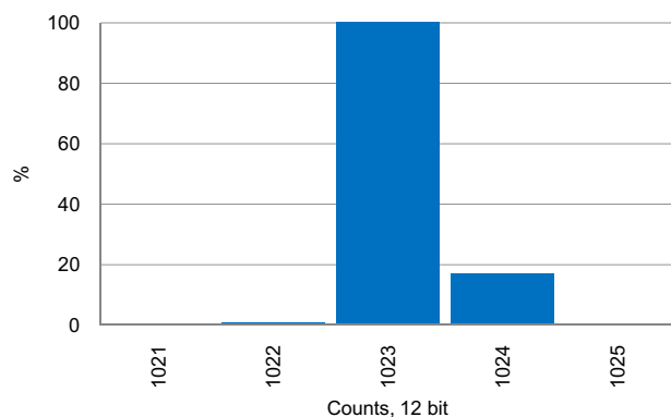
Figure 11-25. SAR ADC Noise Histogram, 100 kps, Internal Reference No Bypass
