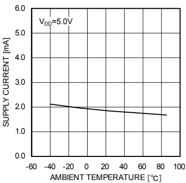
Fig.56 I_{DD} – Ambient temperature
