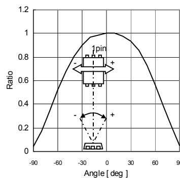
Fig.5 Directional Characteristics 1
