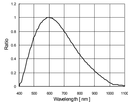
Fig.1 Spectral Response of Type0 (visible light peak)
