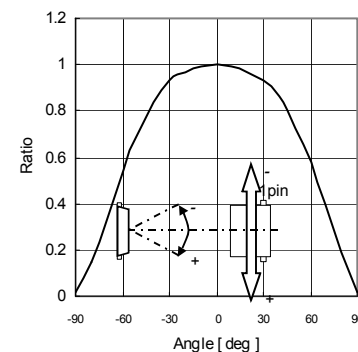
Fig.6 Directional Characteristics 2
