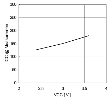
Fig.9 VCC - ICC (During measurement)
