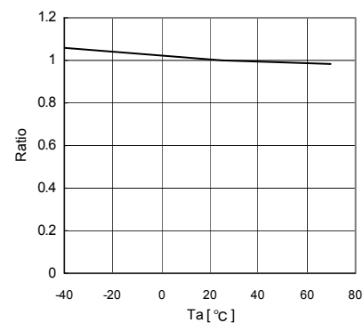
Fig.7 ADC count value in Type0 Temperature Dependency
