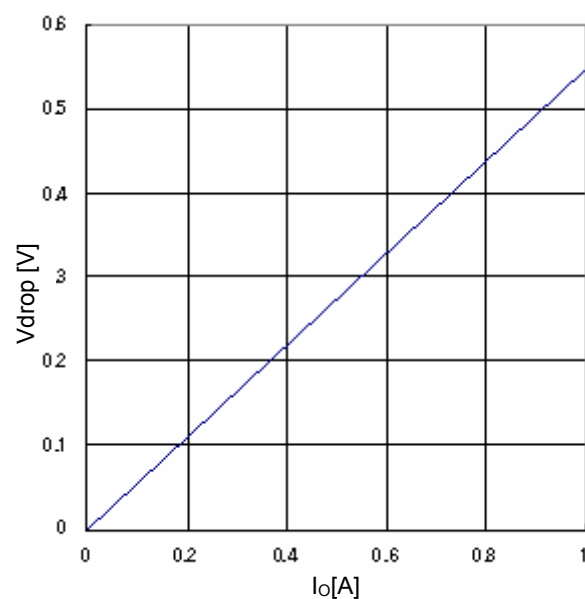
Fig.22 Minimum dropout Voltage 2 ( V_{CC}=4.5 V, T_a=25^{\circ}\text{C} )
