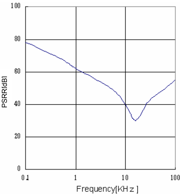
Fig.21 PSRR ( I_o=0mA )
