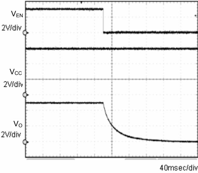
Fig.8 OFF sequence 2 C_o=1\mu F
