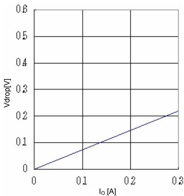
Fig.26 Minimum dropout Voltage 6 ( V_{CC}=12V , T_a=25^\circ C )
