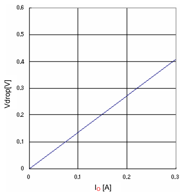
Fig.22 Minimum dropout Voltage 2 ( V_{CC}=4.5 V、 T_a=25^{\circ}\text{C} )
