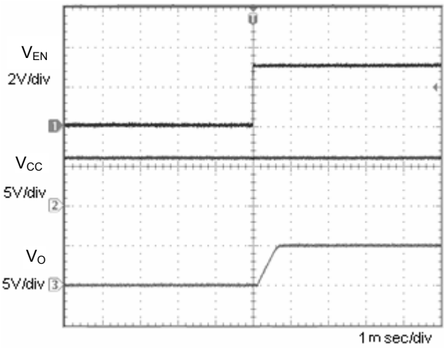
Fig.7 Input sequence 2 C_o=1\mu F
