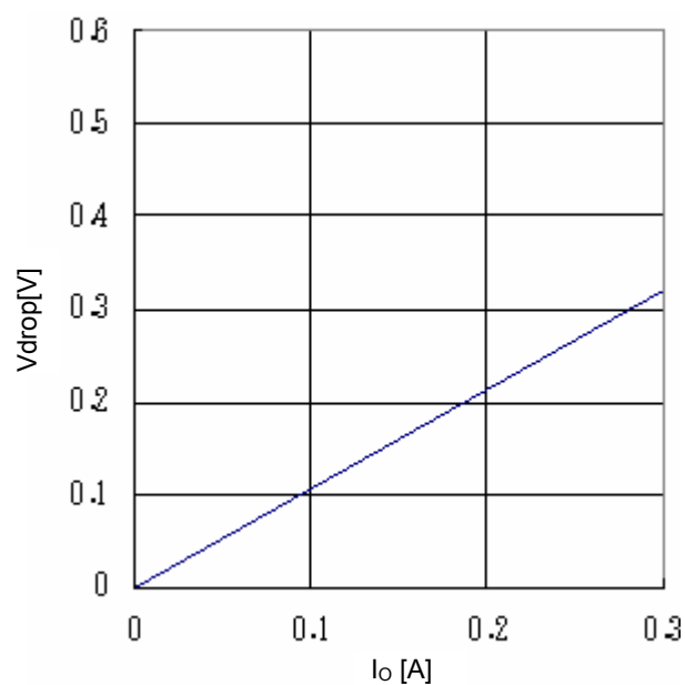
Fig.23 Minimum dropout Voltage 3 ( V_{CC}=6V , T_a=25^\circ C )
