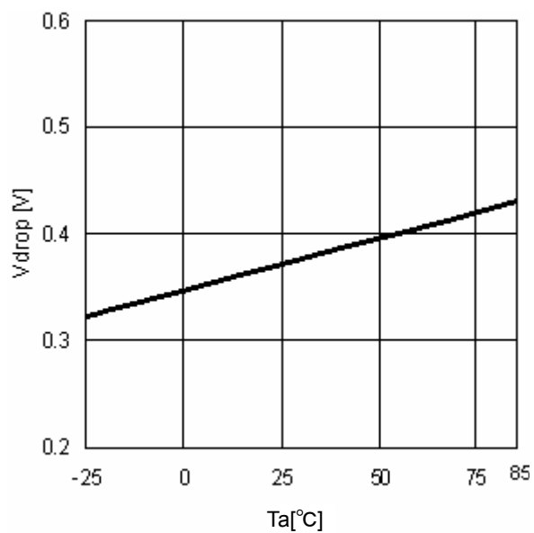
Fig. 18 Minimum dropout Voltage1 ( V_{CC}=5\text{V} , I_O=0.3\text{A} )
