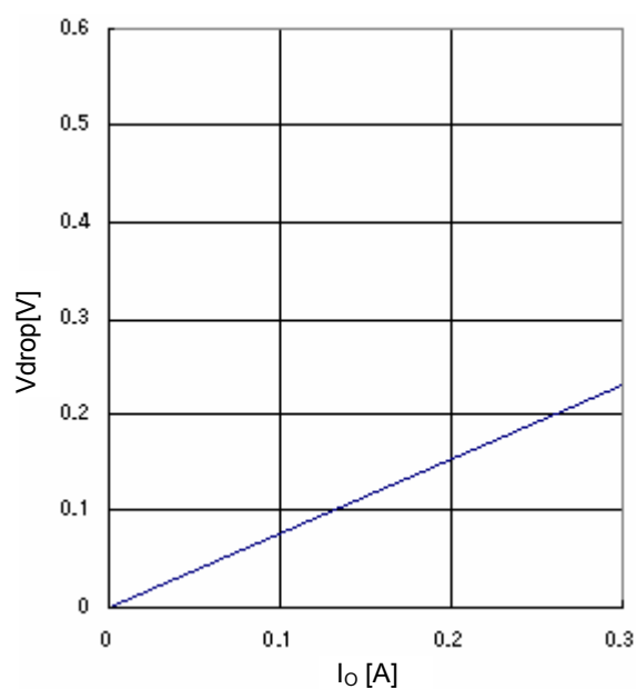
Fig.25 Minimum dropout Voltage 5 ( V_{CC}=10V , T_a=25^\circ C )
