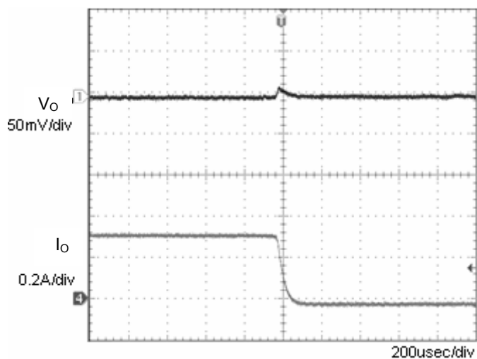
Fig.4 Transient Response (0.3→0A) C_o=1\mu\text{F}
