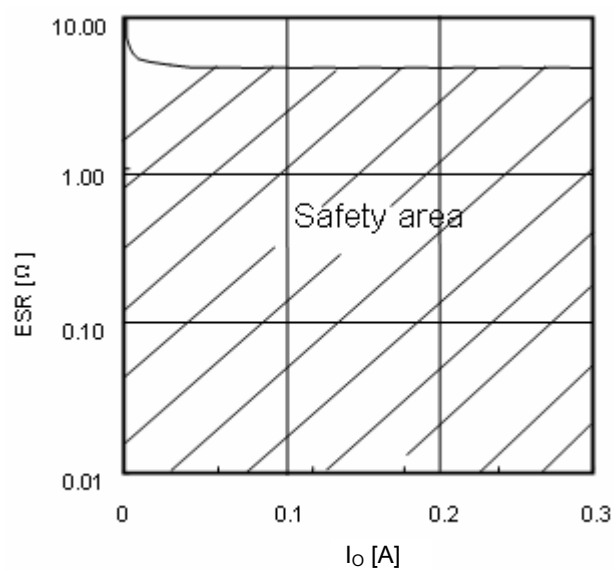
Fig.19 Operation Safety area
