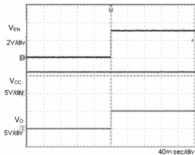
Fig.5 Input sequence 1 C_o=1\mu\text{F}
