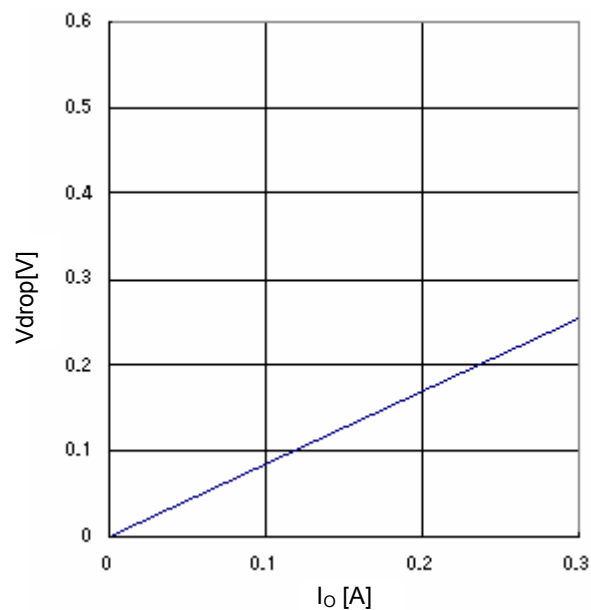
Fig.24 Minimum dropout Voltage 4 ( V_{CC}=8V , T_a=25^\circ C )
