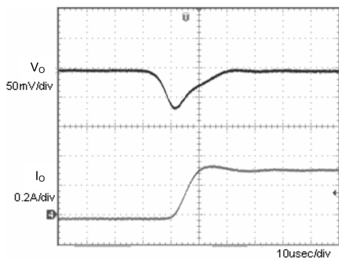
Fig.3 Transient Response (0→0.3A) C_o=1\mu\text{F}
