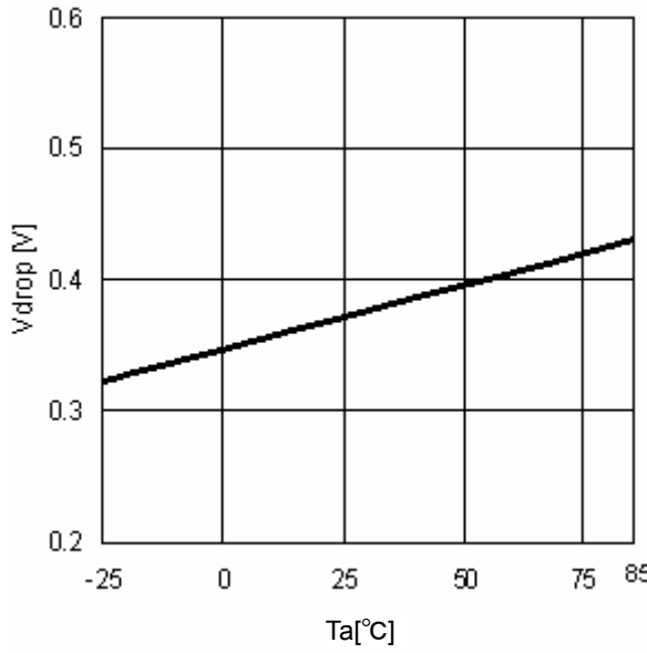
Fig.18 Minimum dropout Voltage1 (V CC =5V, I O =0.3A)
