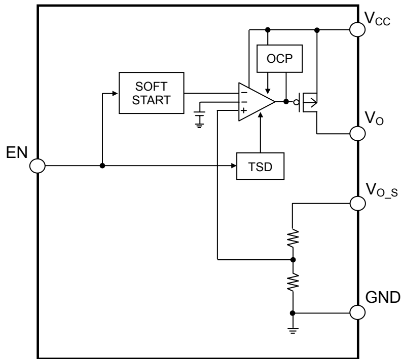
Fig.2 Block Diagram
