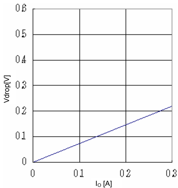
Fig.26 Minimum dropout Voltage 6 ( V_{CC}=12V , T_a=25^\circ C )
