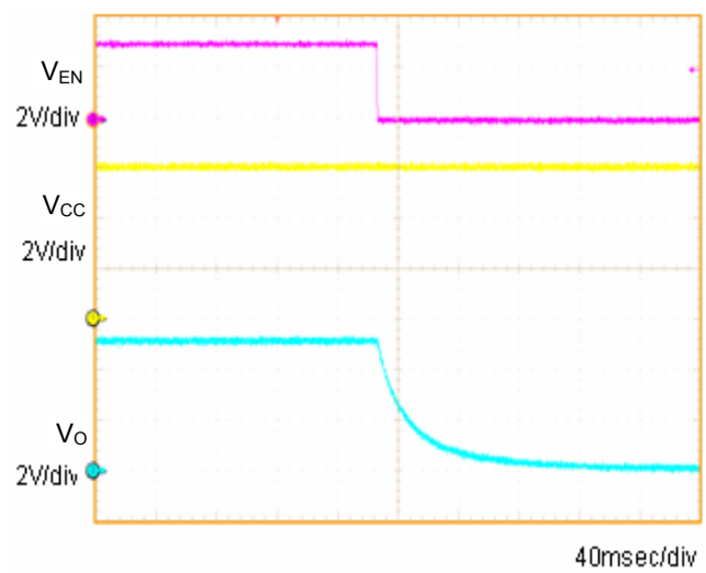
Fig.8 OFF sequence 2 C_o=1\mu\text{F}
