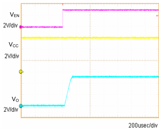
Fig.7 Input sequence 2 C_o=1\mu\text{F}
