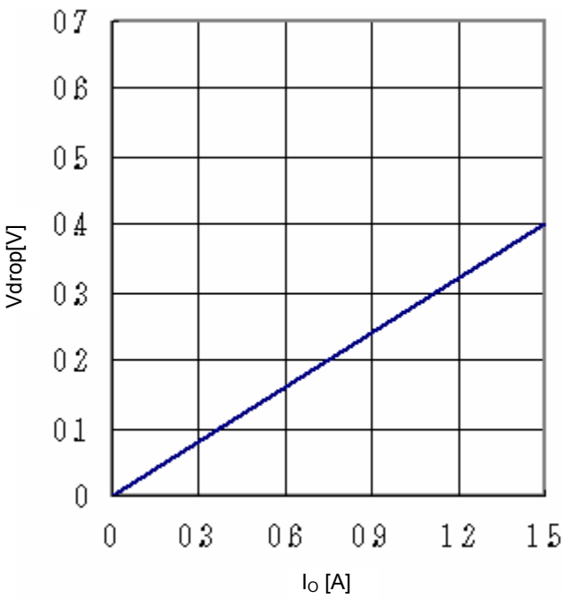
Fig.24 Minimum dropout Voltage 4 (V CC =8V、Ta=25°C)
