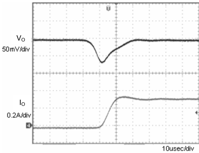
Fig.3 Transient Response (0→0.3A) Co=1µF
