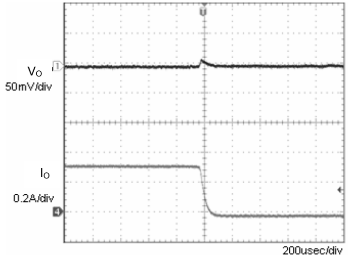
Fig.4 Transient Response (0.3→0A) Co=1µF
