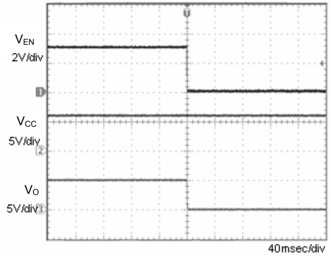
Fig.8 OFF sequence 2 Co=1μF
