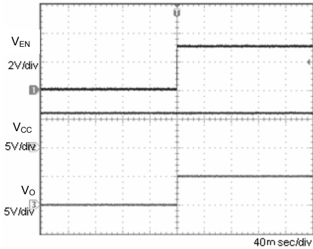
Fig.5 Input sequence 1 Co=1µF
