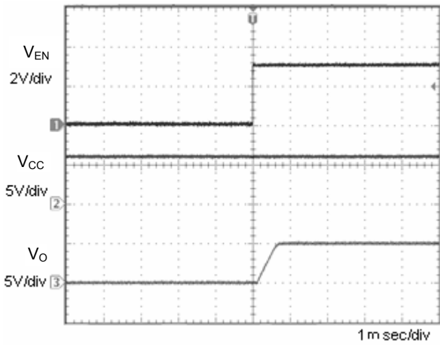
Fig.7 Input sequence 2 Co=1μF
