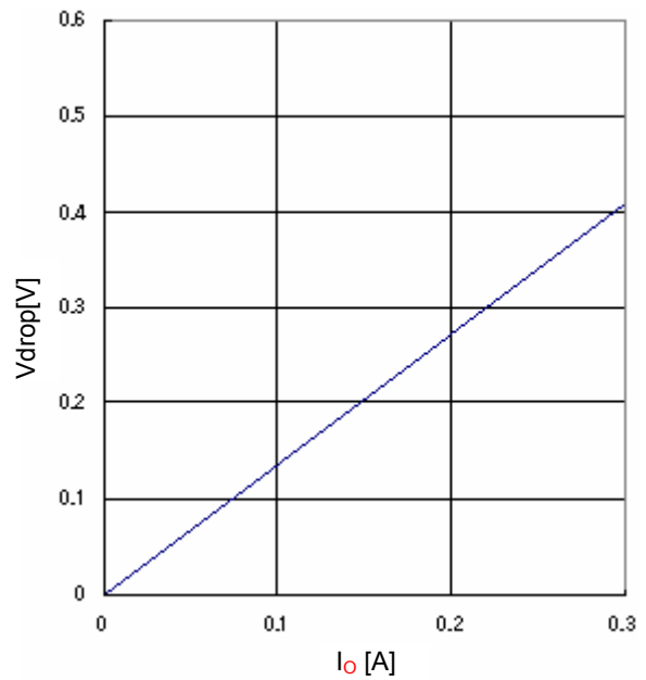
Fig.22 Minimum dropout Voltage 2 (Vcc=4.5V、Ta=25°C)
