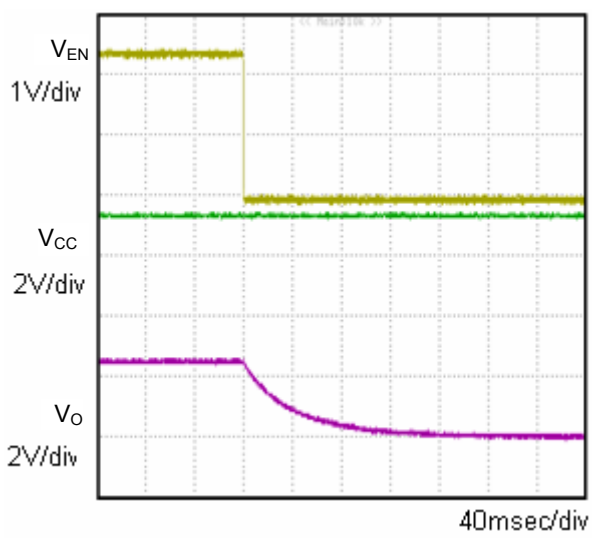
Fig.8 OFF sequence 2 C_o=1\mu F
