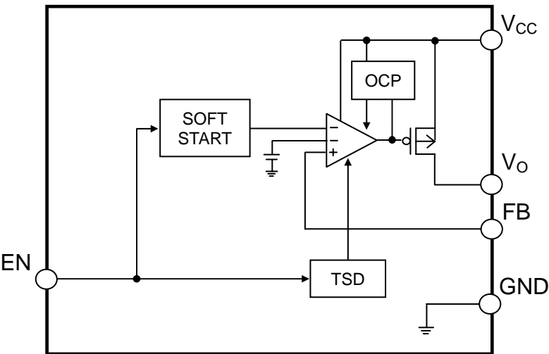
Fig.1 Block Diagram
