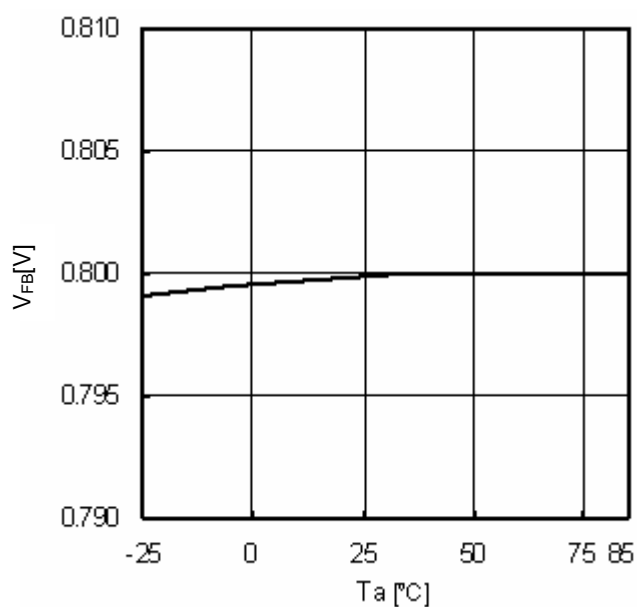
Fig.9 T_a - V_{FB}
