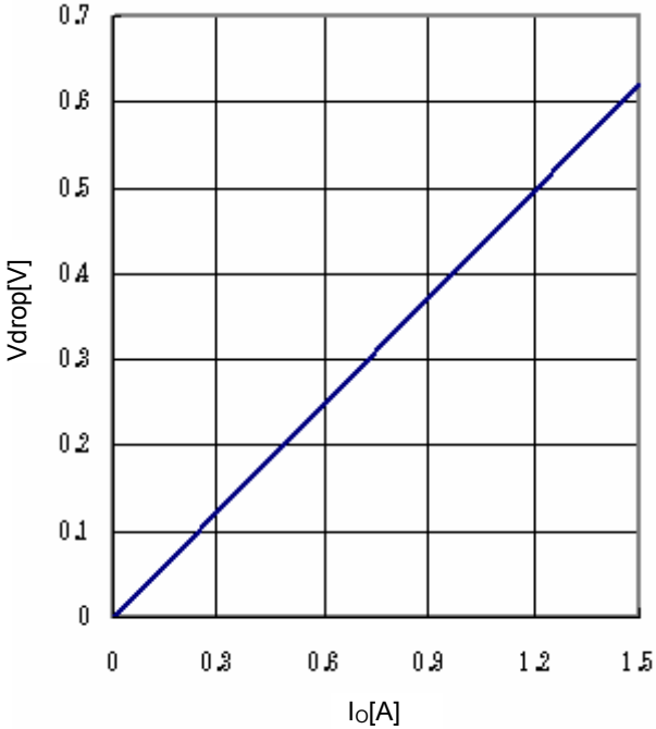
Fig.22 Minimum dropout Voltage 2 ( V_{CC} =4.5V、 T_a =25°C)
