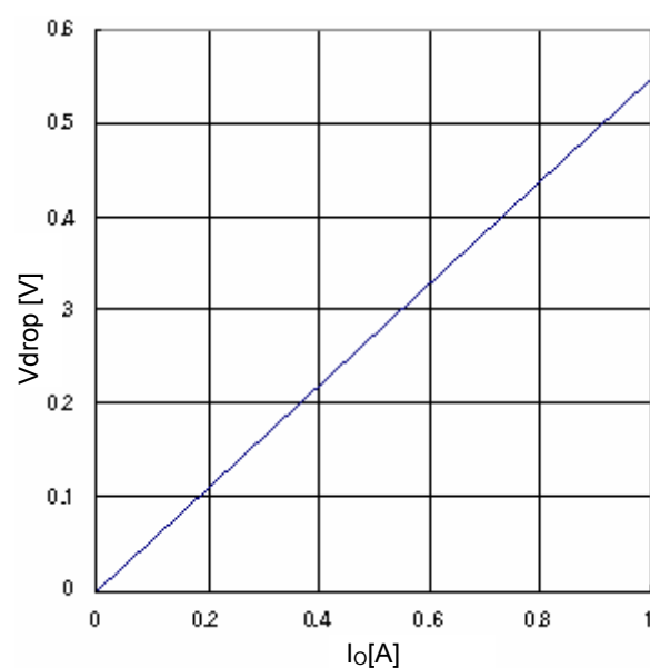
Fig.22 Minimum dropout Voltage 2 ( V_{CC}=4.5V , T_a=25^{\circ}C )
