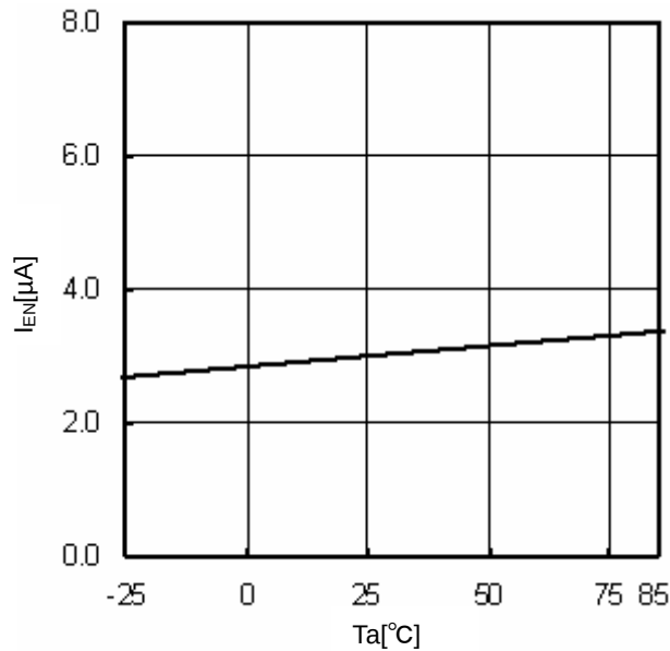
Fig.14 T_a - I_{EN}
