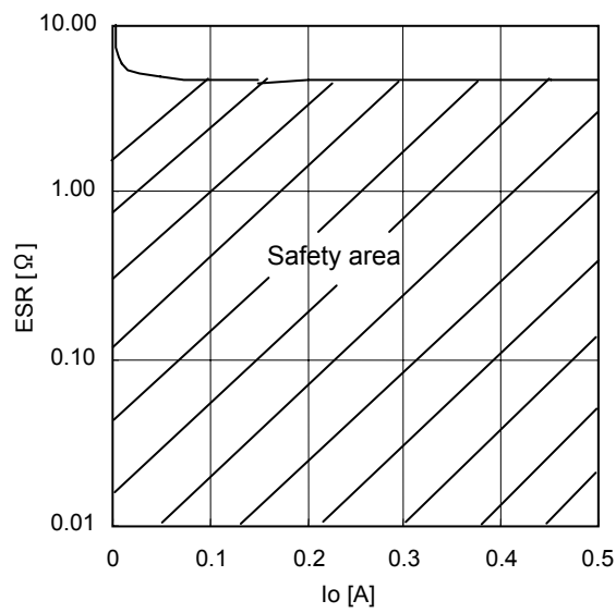
Fig.19 ESR Condencer
