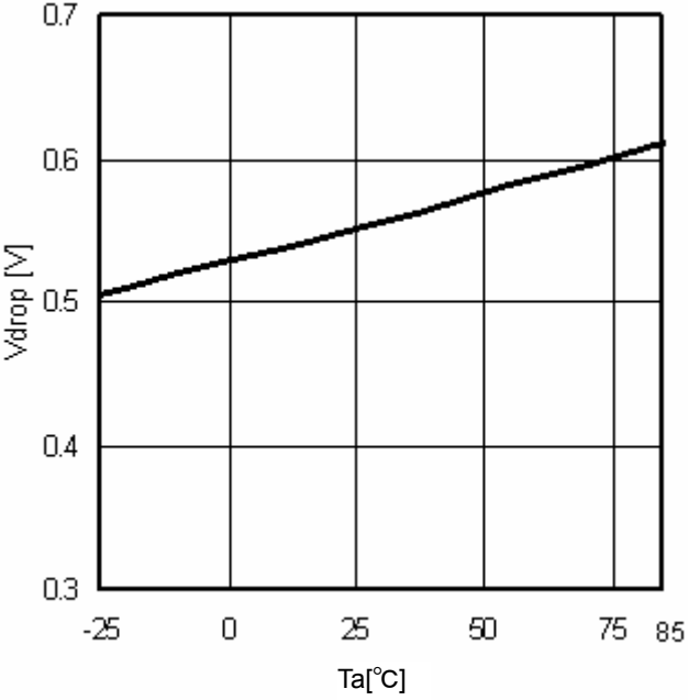
Fig.18 Minimum dropout Voltage1 ( V_{cc}=5V , I_o=-1.5A )
