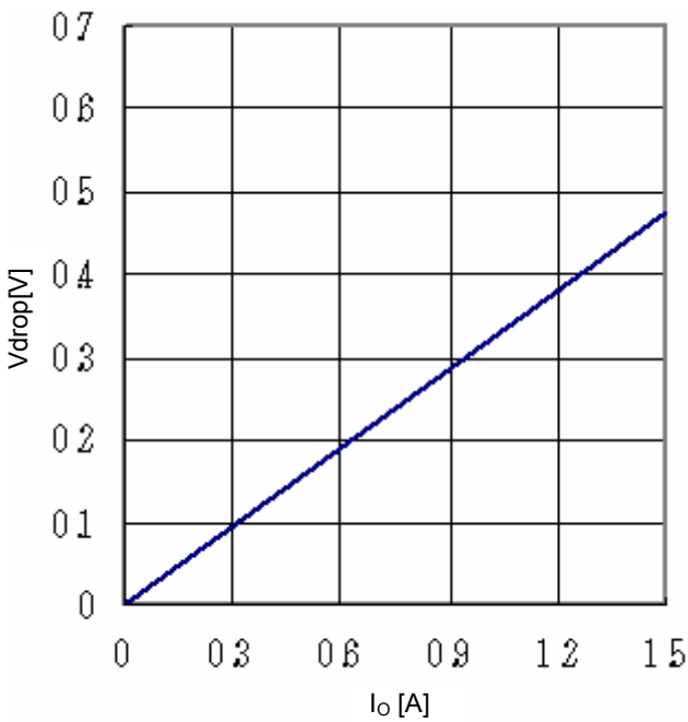
Fig.23 Minimum dropout Voltage 3 ( V_{CC}=6V 、 T_a=25^\circ C )
