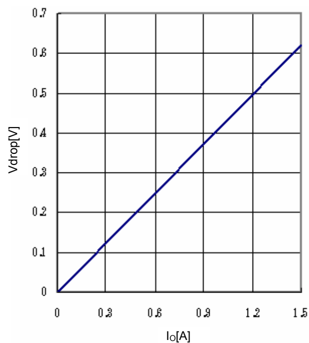
Fig.22 Minimum dropout Voltage 2 ( V_{CC}=4.5 V, T_a=25^{\circ} C)
