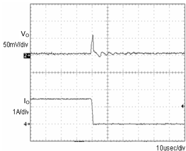
Fig.4 Transient Response (1.5→0A) C_o=1\mu\text{F}
