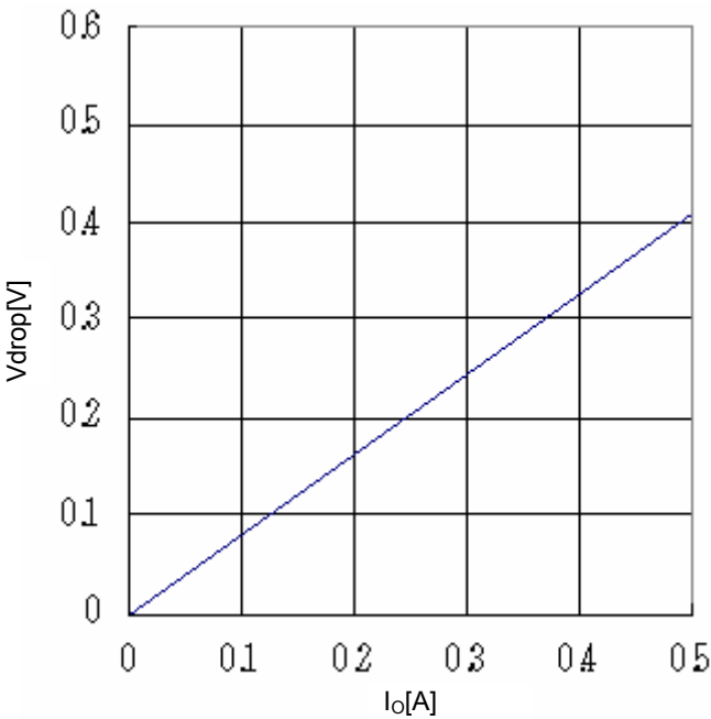
Fig.22 Minimum dropout Voltage 2 ( V_{cc}=4.5\text{V} , T_a=25^\circ\text{C} )
