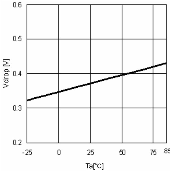
Fig.18 Minimum dropout Voltage1 ( V_{CC}=5V , I_O=0.3A )
