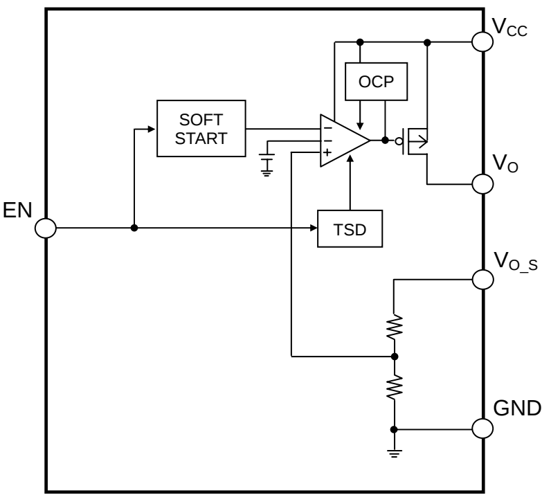
Fig.2 Block Diagram
