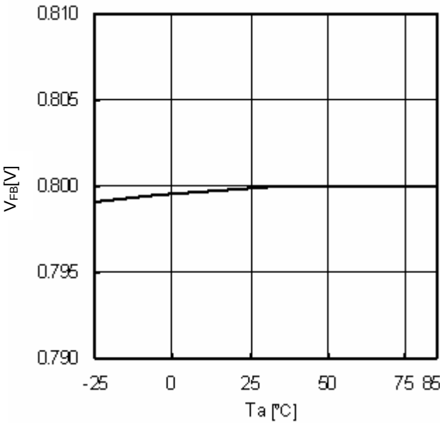
Fig.9 T a -V FB
