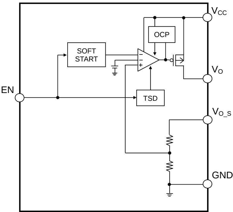
Fig.2 Block Diagram
