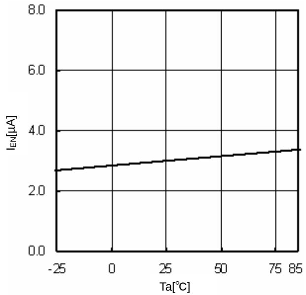
Fig.14 T_a - I_{EN}
