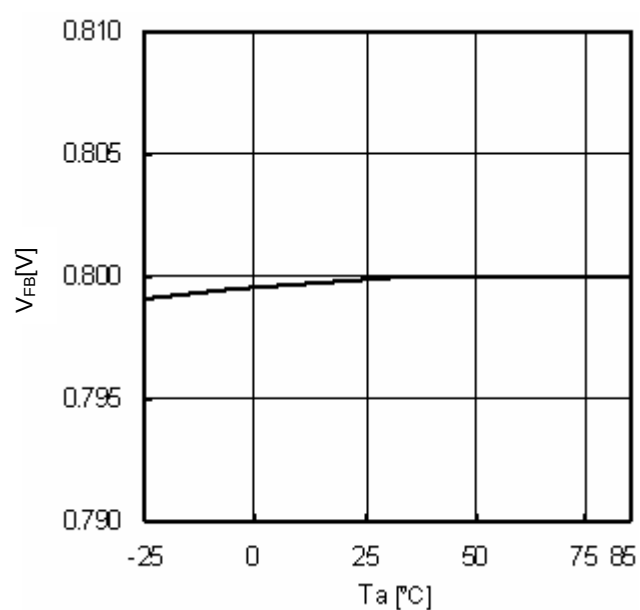
Fig.9 T_a - V_{FB}
