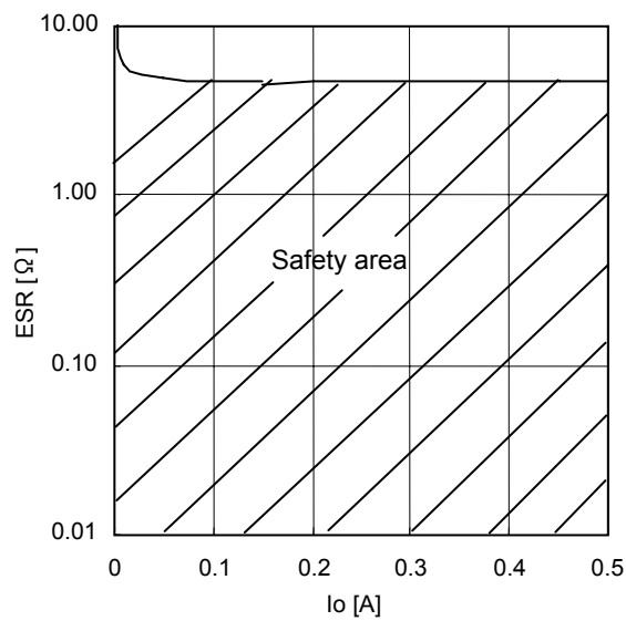
Fig.19 ESR Condencer
