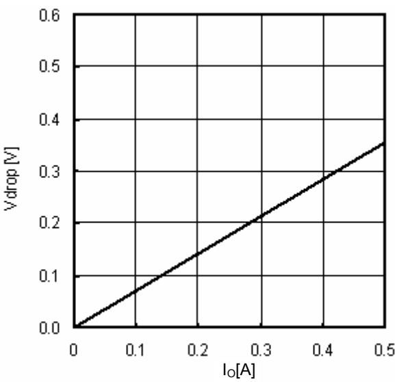
Fig.24 Minimum dropout Voltage 4 (VCC=5.0V, Ta=25°C)
