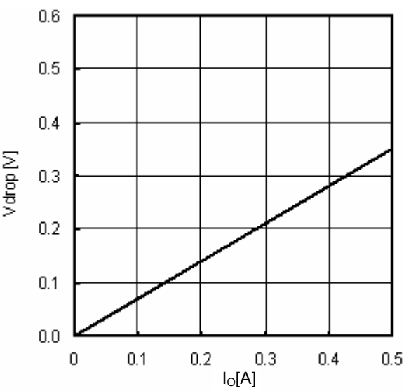
Fig.23 Minimum dropout Voltage 3 (VCC=3.3V, Ta=25°C)
