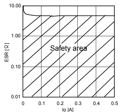
ESR – I_O characteristics
