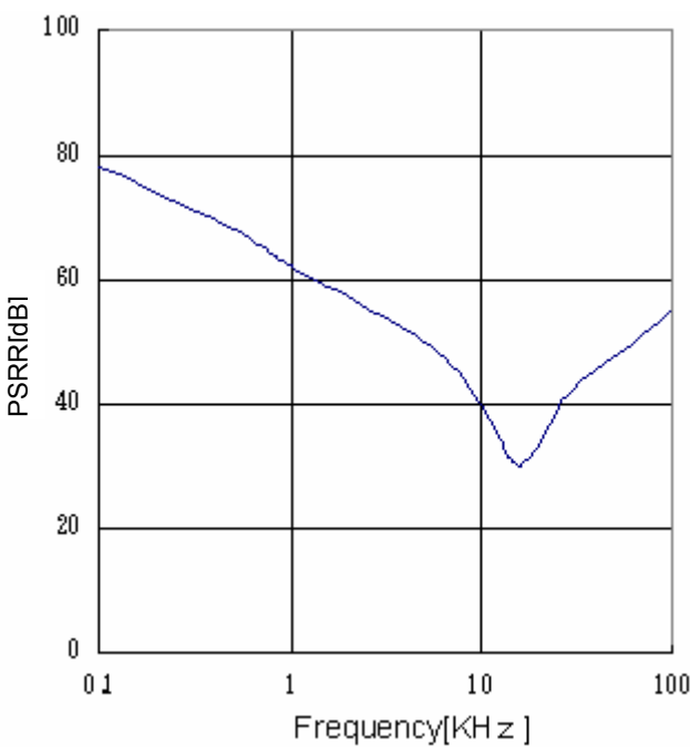
Fig.21 PSRR ( I_o=0mA )
