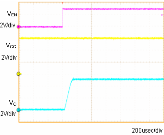
Fig.7 Input sequence 2 Co=1µF
