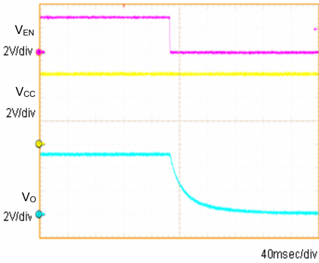
Fig.8 OFF sequence 2 Co=1µF
