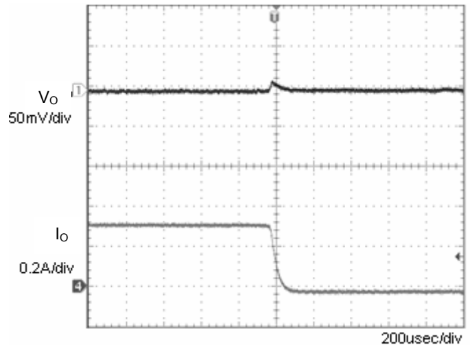
Fig.4 Transient Response (0.3→0A) C_o=1\mu\text{F}
