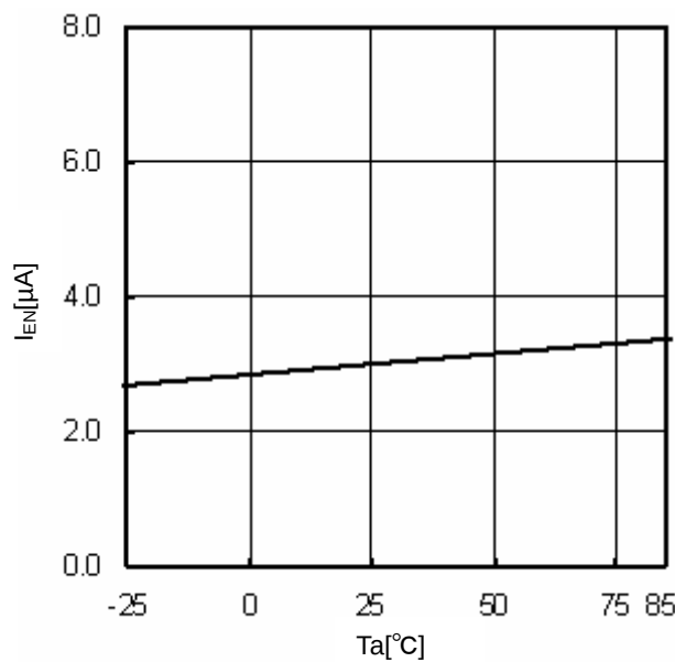
Fig.14 T_a - I_{EN}
