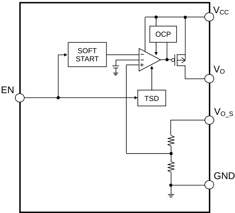
Fig.2 Block Diagram
