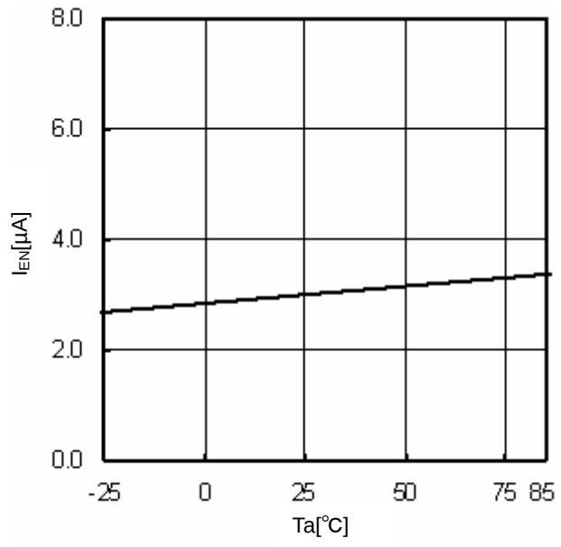
Fig.14 T_a - I_{EN}
