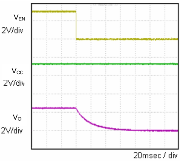
Fig.8 OFF sequence 2 Co=1.0μF
