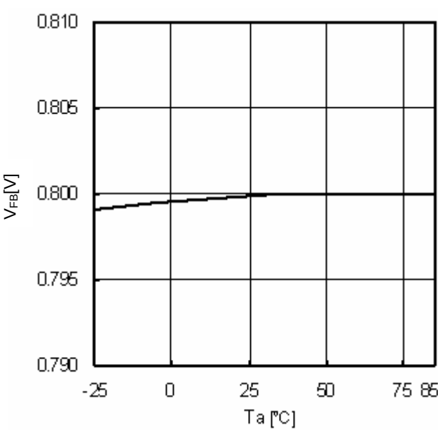
Fig.9 T a -V FB
