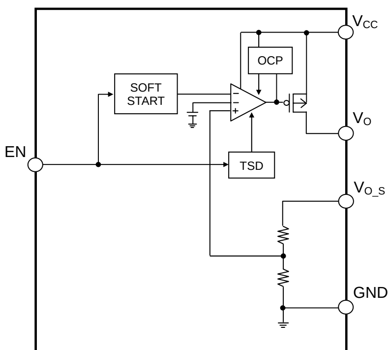
Fig.2 Block Diagram
