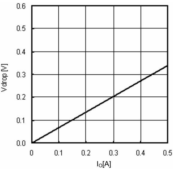
Fig.22 Minimum dropout Voltage 2 (VCC=2.4V, Ta=25°C)
