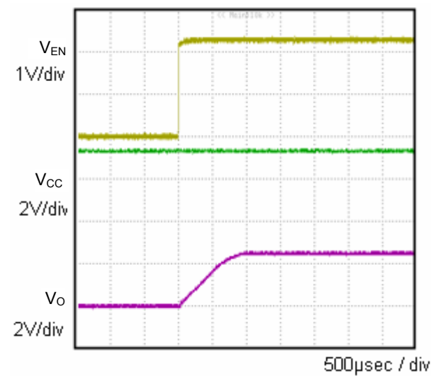
Fig.7 Input sequence 2 Co=1μF
