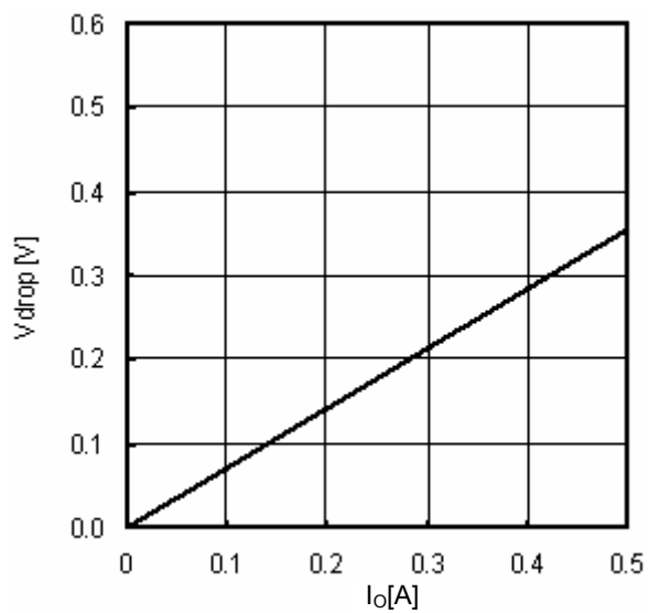
Fig.24 Minimum dropout Voltage 4 ( V_{CC}=5.0V , T_a=25^{\circ}C )
