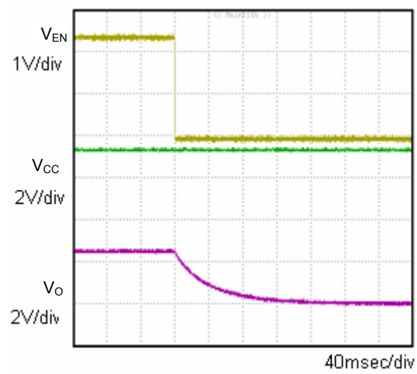
Fig.8 OFF sequence 2 Co=1μF
