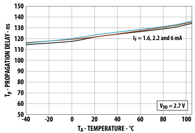
Figure 8. Propagation Delay, t_{PHL} vs. Temperature
