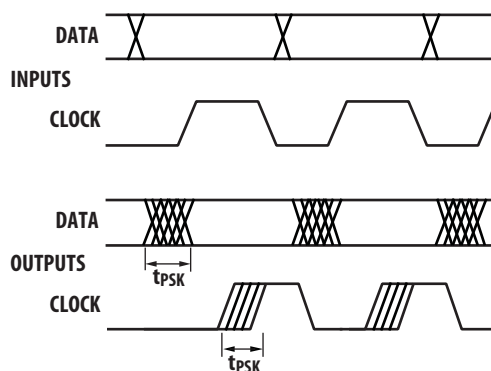
Figure 11. Parallel data transmission example
