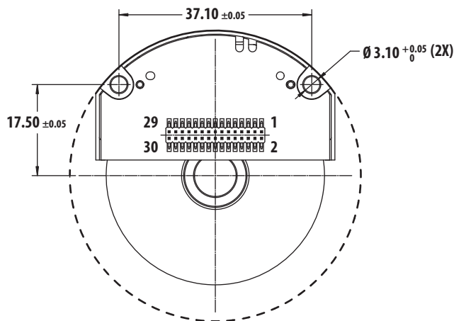
Figure 2. Alignment between read heard and the codewheel.
