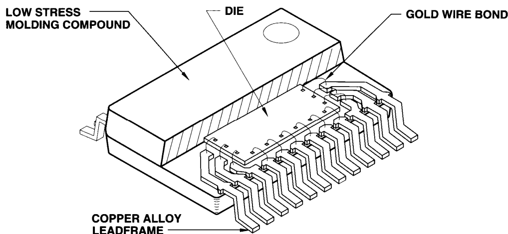
Figure 25: SSOP Package
