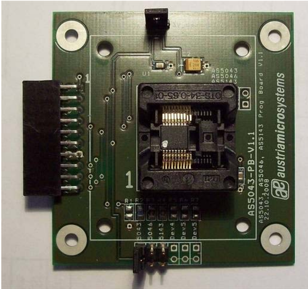
AS5043 10-bit Programmable Angle Magnetic Rotary Encoder with Absolute Digital and Analog Outputs Programming Board
