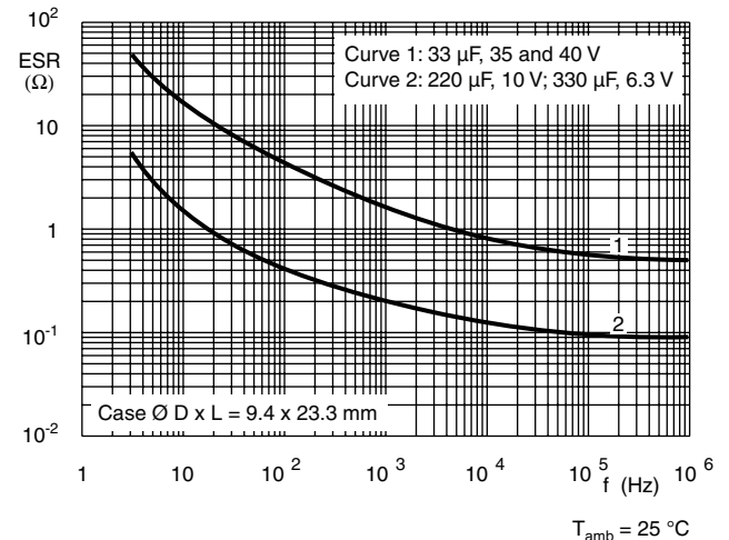
Fig.27 Typical ESR as a function of frequency
