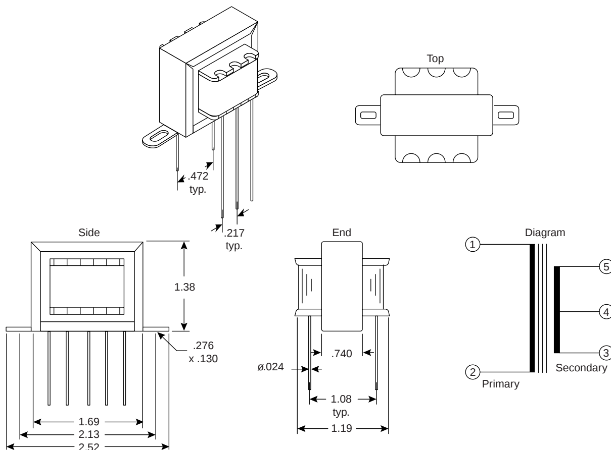
Dimensions (In.)
