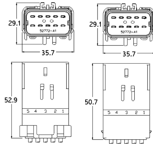
Sealed Assembly
