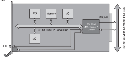
Typical Compact PCI Hot Swap Adapter Card
